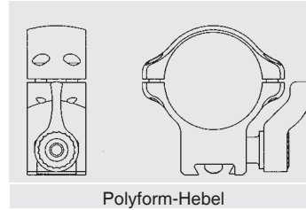
Polyform-Hebel
